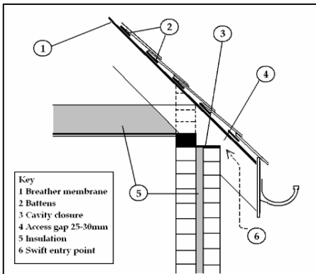
Typical Open Soffit Construction © RSPB / Action for Swifts
